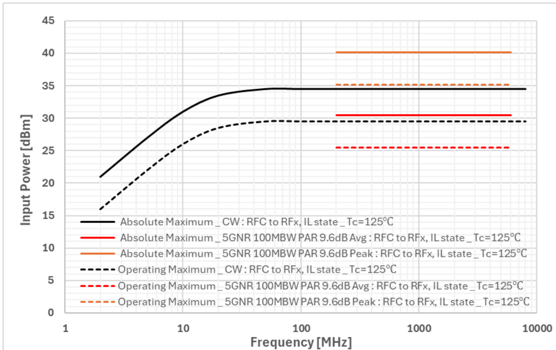
Figure 4. Power De-rating Curve
