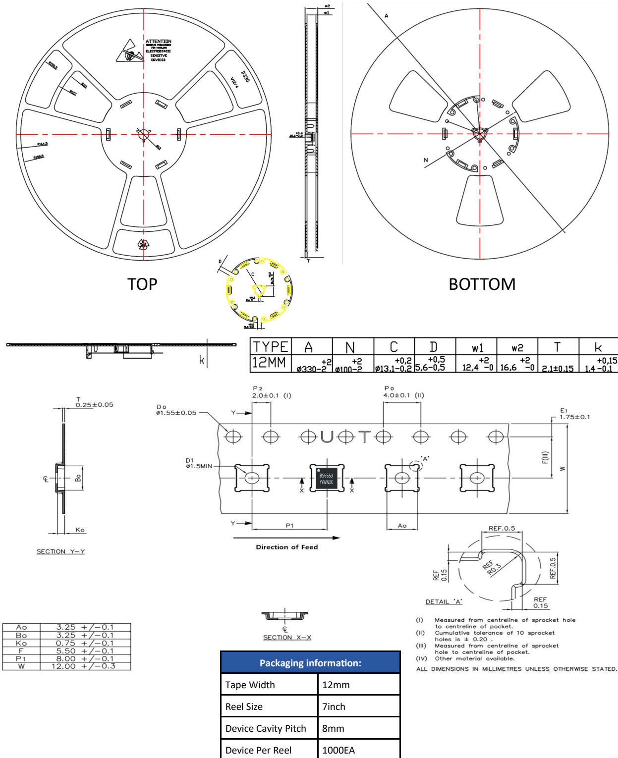
Figure 33. Tape & Reel
