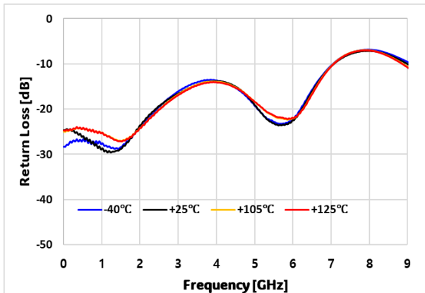
Figure 13. Return Loss vs Temp (Active Port)
