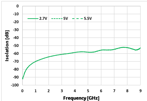
Figure 23. Isolation vs VDD (RF1 to RF2, RF1 ON)
