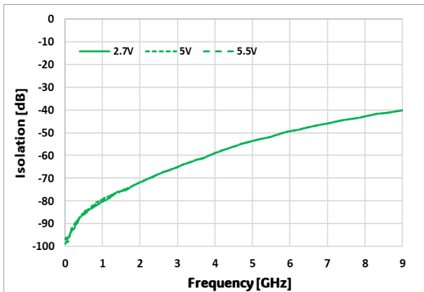
Figure 19. Isolation vs VDD (RFC to RF1, RF2 ON)
