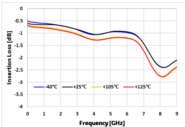
Figure 7. Insertion Loss vs Temp (RFC-RF1)
