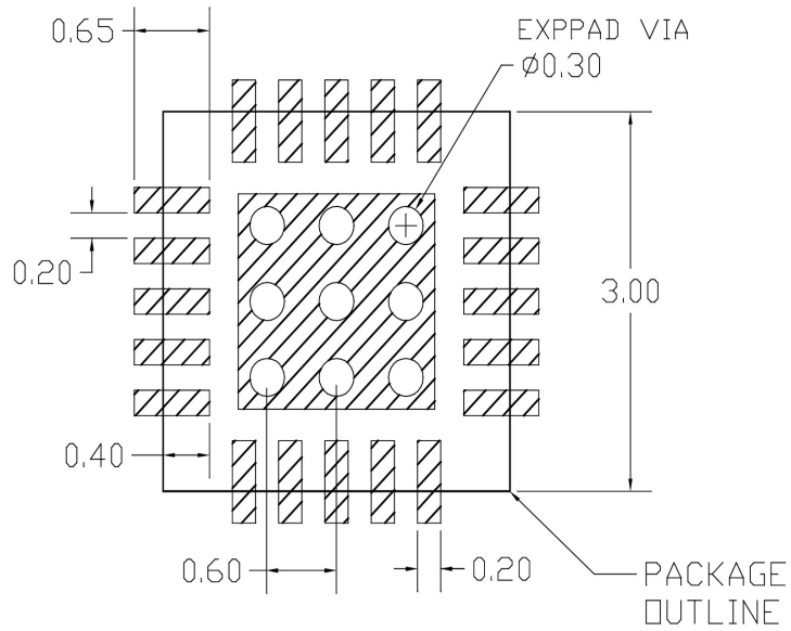
Figure 31. Recommended Land Pattern
