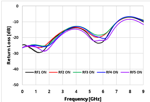
Figure 1 Return Loss vs Frequency (Active Port)
