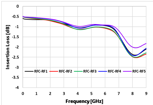
Figure 5. Insertion Loss vs Frequency
