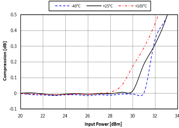
Figure 31. Input 0.1dB Compression vs Temp. @ 5500MHz
