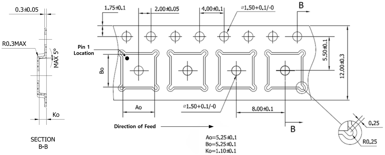
Figure 66. Tape & Reel
