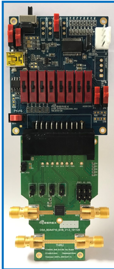
Figure 58. BDA4710 EVK
