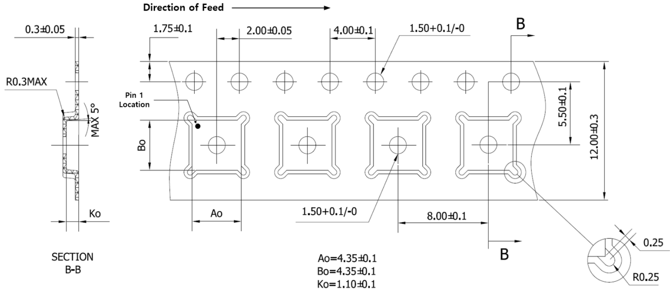
Figure 57. Tape & Reel
