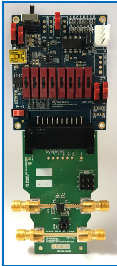
Figure 49. BDA4630 EVK
