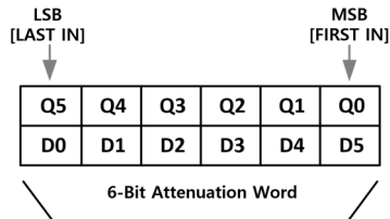
Figure 6. Serial Register Map
