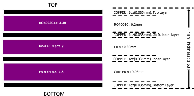
Figure 52. Evaluation Board PCB Layer Information
