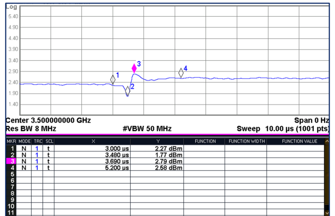
Figure 34. ATT Transient (16 to 15.5dB, Pin=18dBm)
