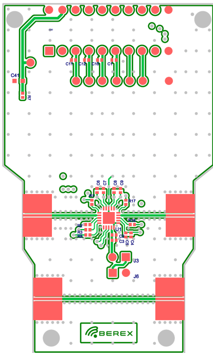
Figure 31. Evaluation Board PCB Layout Information
