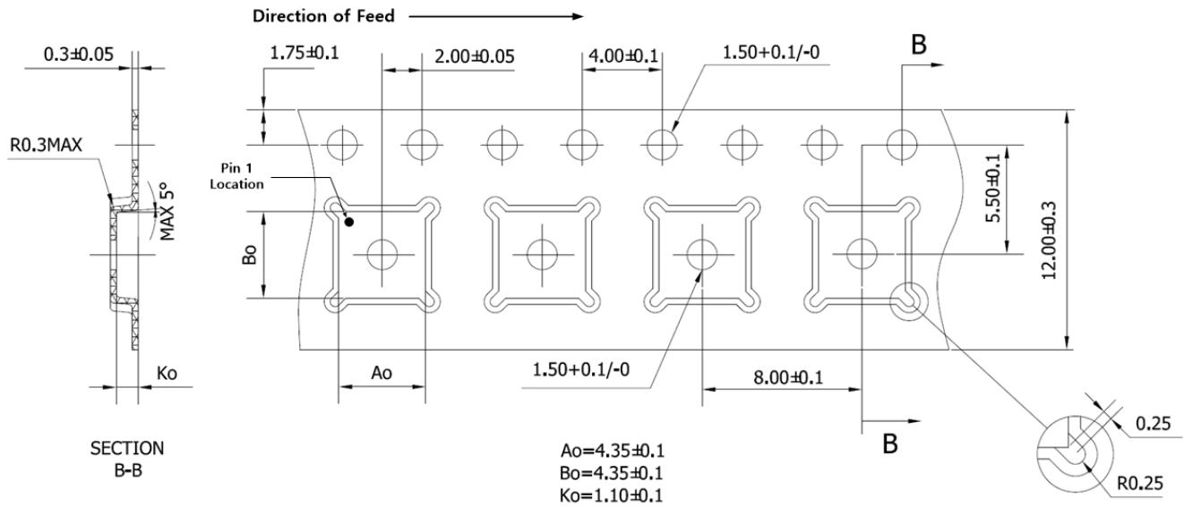
Figure 38. Tape & Reel
