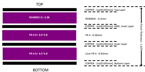
Figure 32. Evaluation Board PCB Layer Information
