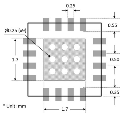
Figure 7. 8TR6113 PCB Layout Footprint
