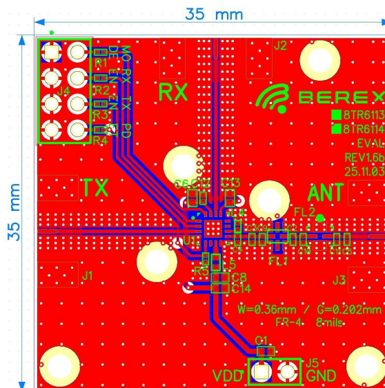
Figure 5. 8TR6113 Evaluation Board PCB Layout
