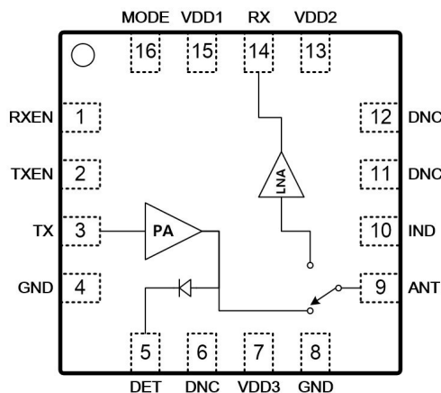
Figure 1. 8TR6113 Functional Block Diagram
