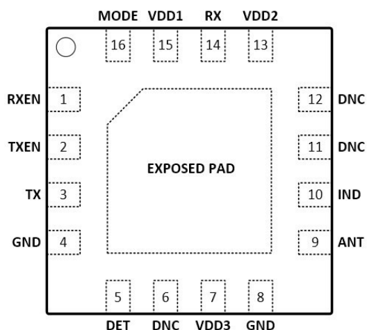
Figure 3. 8TR6113 Pinout (Top View)
