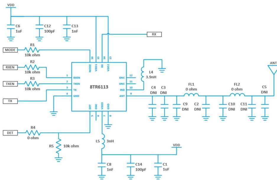
Figure 4. 8TR6113 Evaluation Board Schematic
