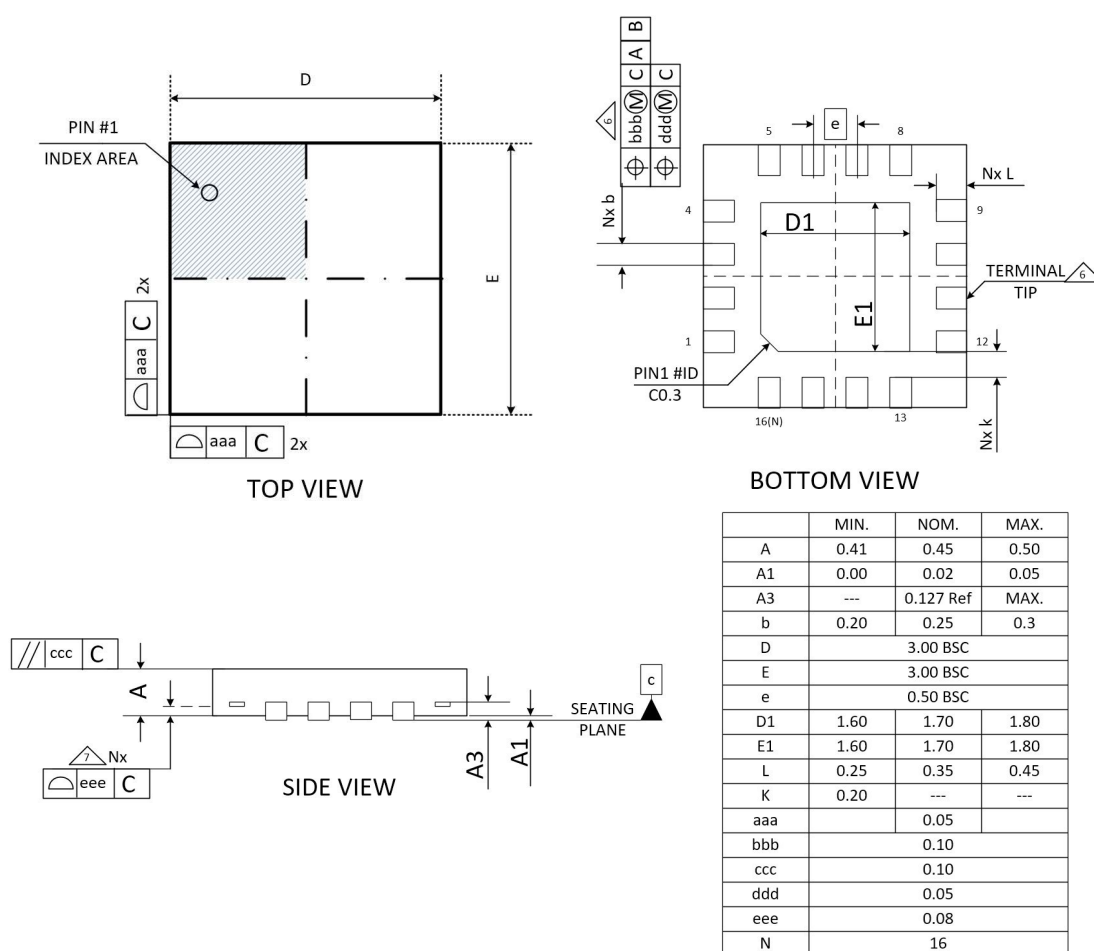
Figure 8. 8TR6113 Package Dimension
